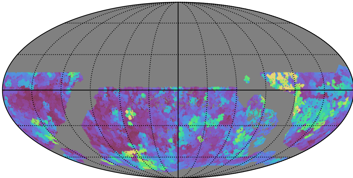
too_elab_r128_d2_gz_v3.4_10yrs WFD g band: Max seeingEff
