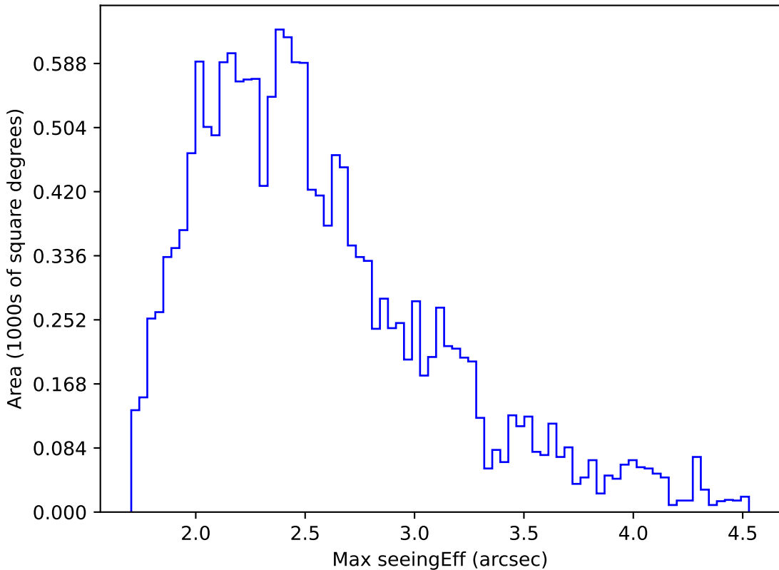
too_elab_r128_d2_gz_v3.4_10yrs WFD g band: Max seeingEff
