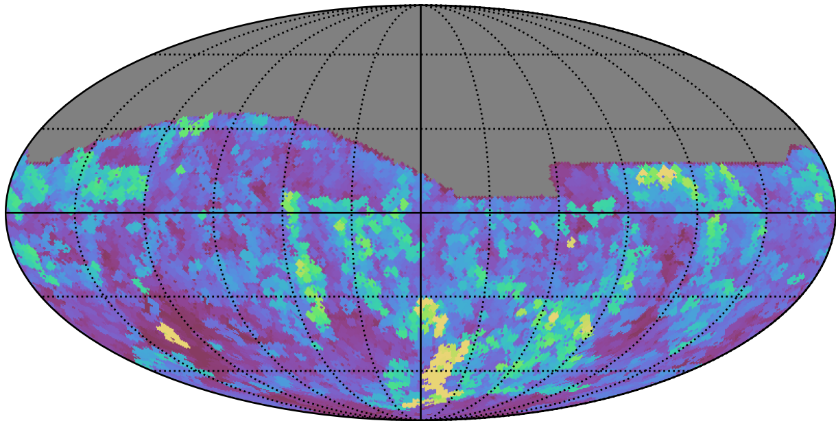
too_elab_r128_d2_gz_v3.4_10yrs All sky z band: Max seeingEff
