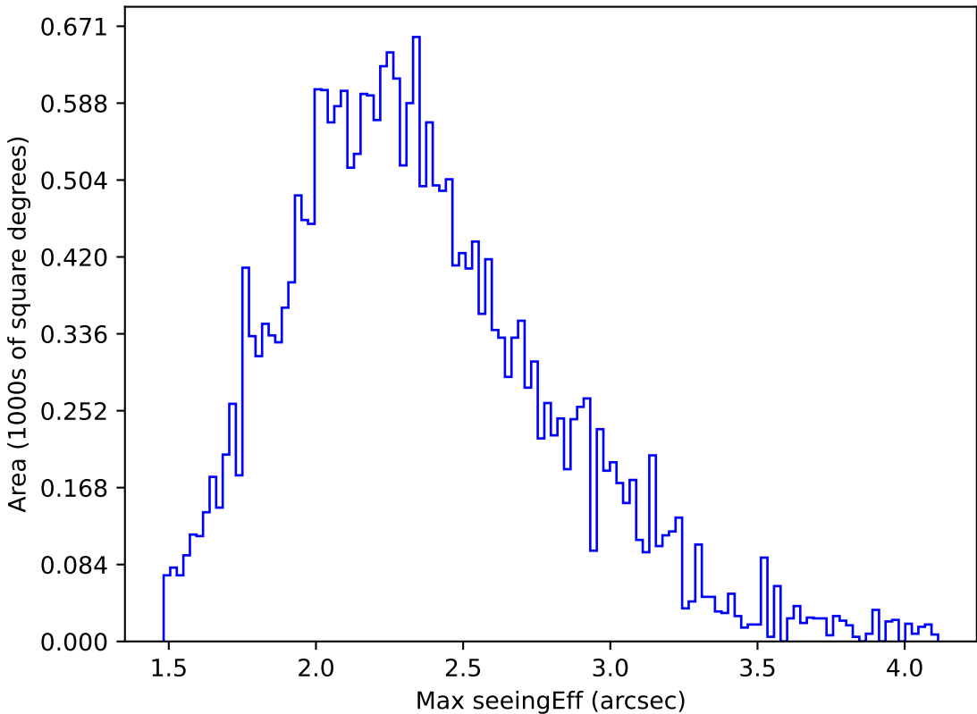
too_elab_r128_d2_gz_v3.4_10yrs All sky z band: Max seeingEff
