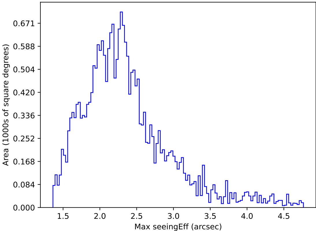
too_elab_r128_d2_gz_v3.4_10yrs All sky y band: Max seeingEff
