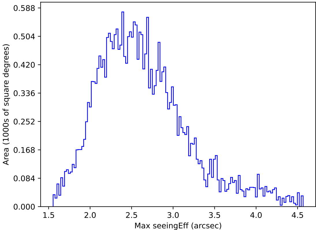
too_elab_r128_d2_gz_v3.4_10yrs All sky r band: Max seeingEff
