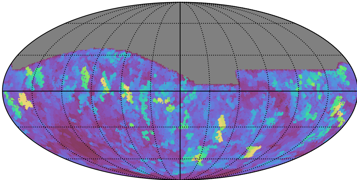
too_elab_r128_d2_gz_v3.4_10yrs All sky i band: Max seeingEff
