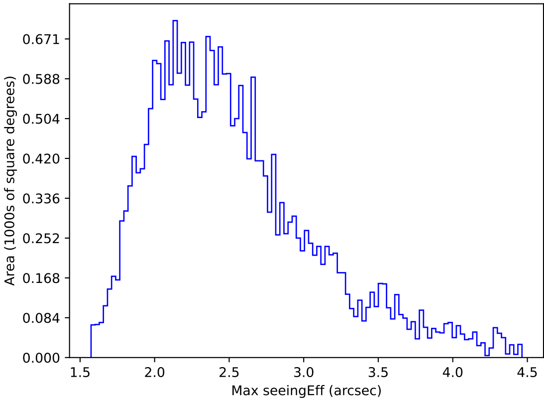
too_elab_r128_d2_gz_v3.4_10yrs All sky g band: Max seeingEff
