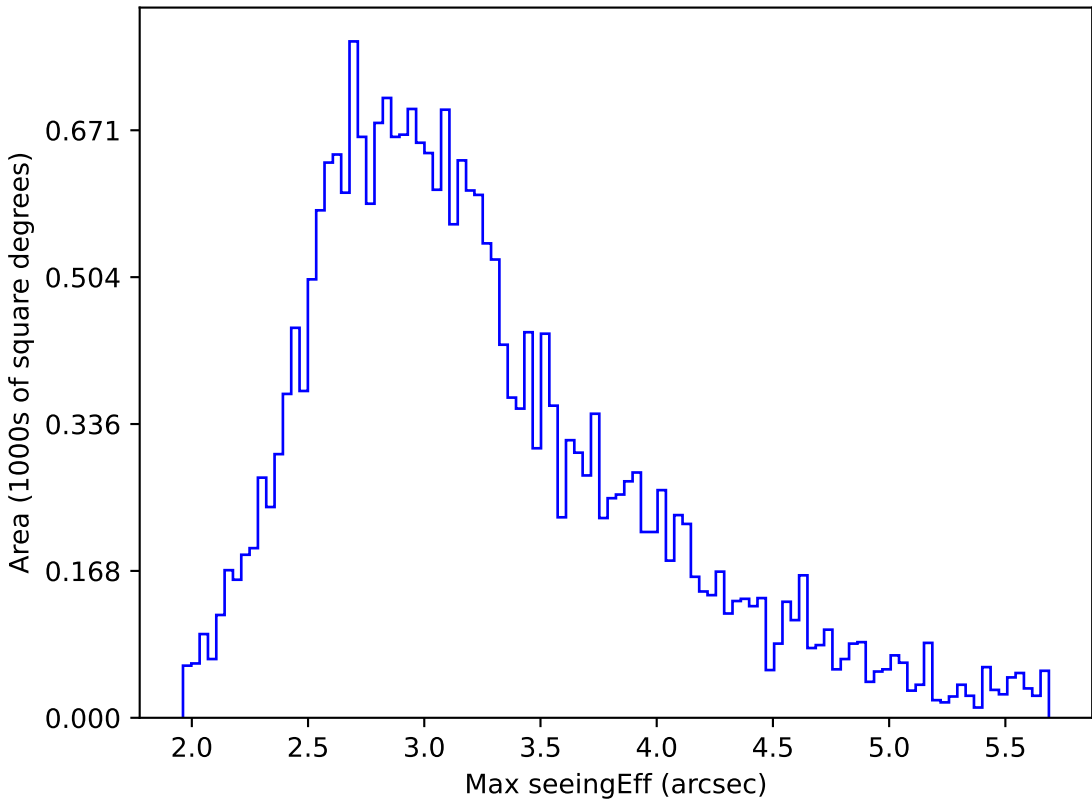
too_elab_r128_d2_gz_v3.4_10yrs All sky all bands: Max seeingEff
