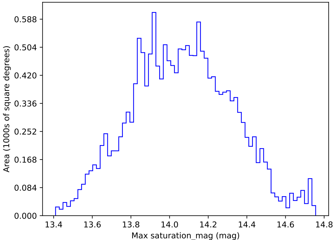
too_elab_r128_d2_gz_v3.4_10yrs WFD u band: Max saturation_mag
