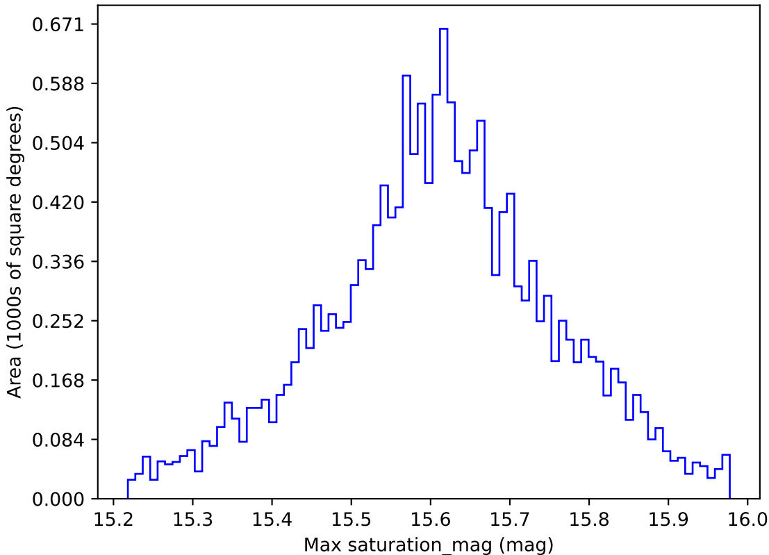
too_elab_r128_d2_gz_v3.4_10yrs WFD i band: Max saturation_mag
