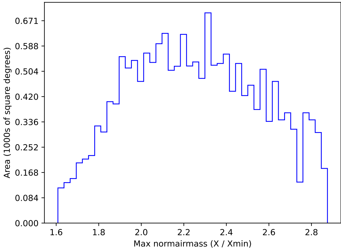
too_elab_r128_d2_gz_v3.4_10yrs WFD z band: Max normairmass
