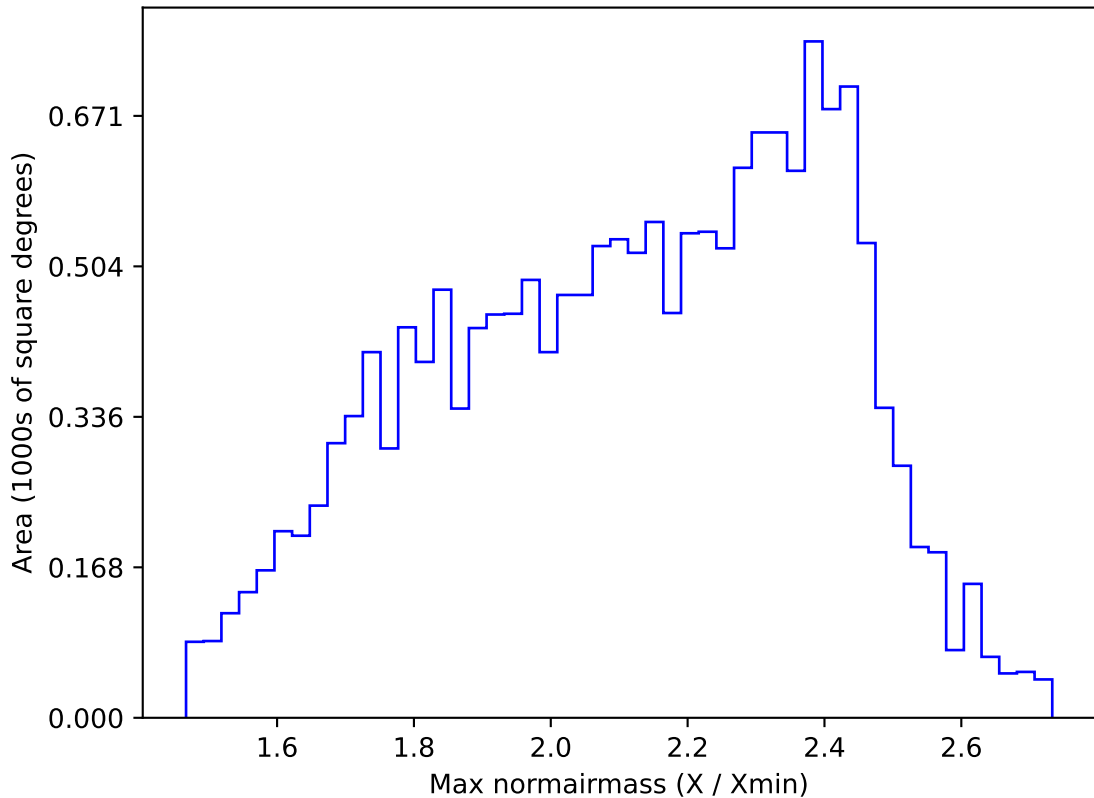
too_elab_r128_d2_gz_v3.4_10yrs WFD r band: Max normairmass
