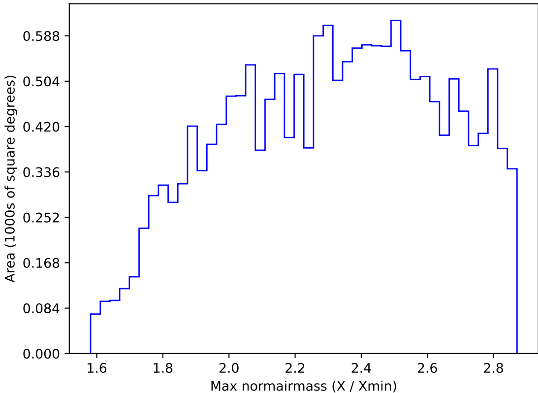
too_elab_r128_d2_gz_v3.4_10yrs WFD i band: Max normairmass
