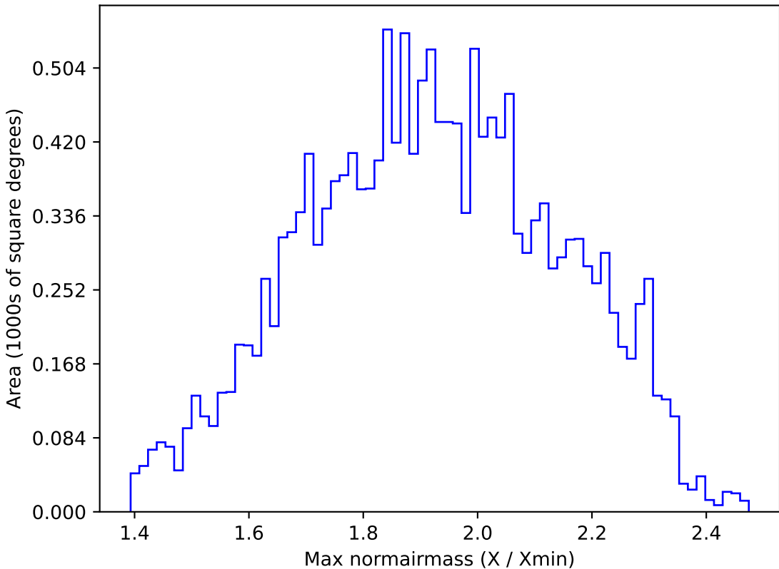
too_elab_r128_d2_gz_v3.4_10yrs WFD g band: Max normairmass
