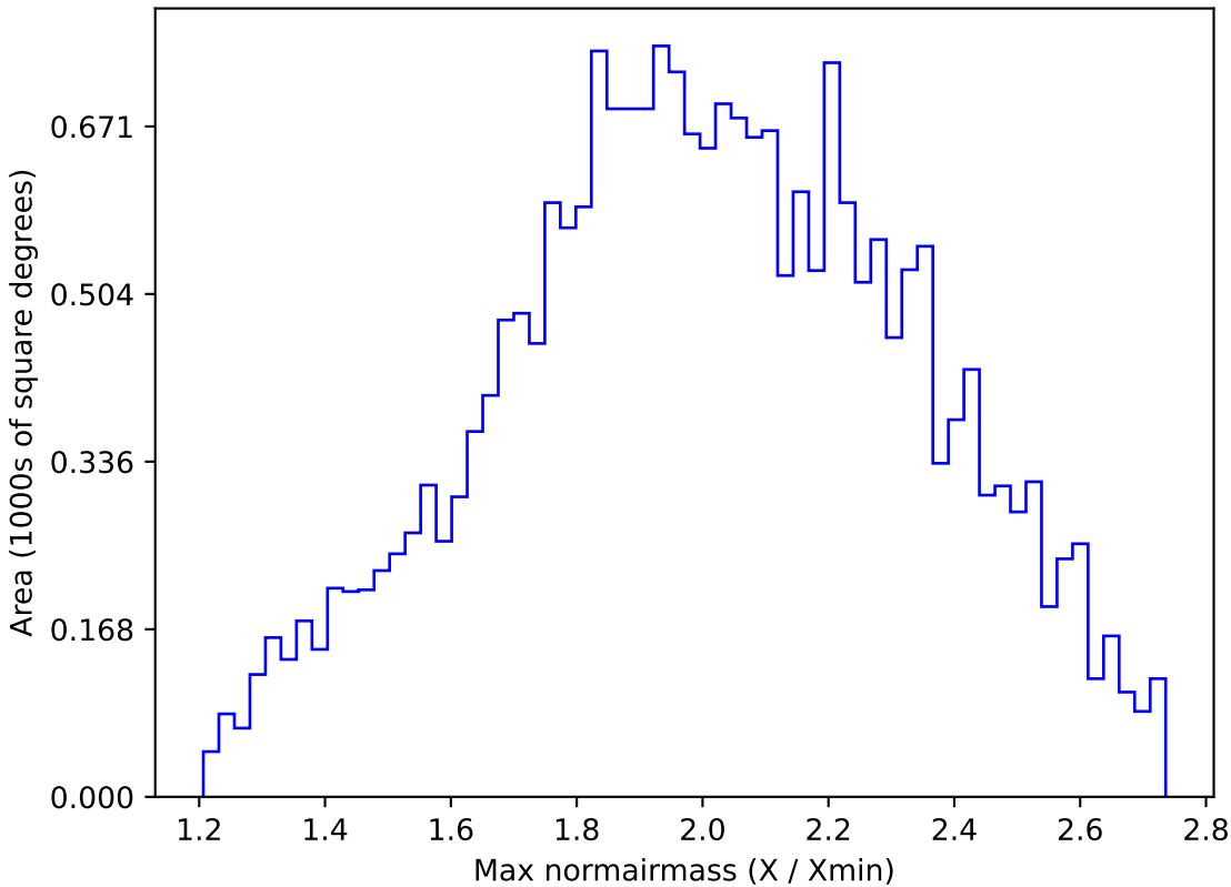
too_elab_r128_d2_gz_v3.4_10yrs All sky y band: Max normairmass
