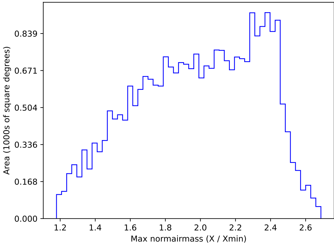
too_elab_r128_d2_gz_v3.4_10yrs All sky r band: Max normairmass
