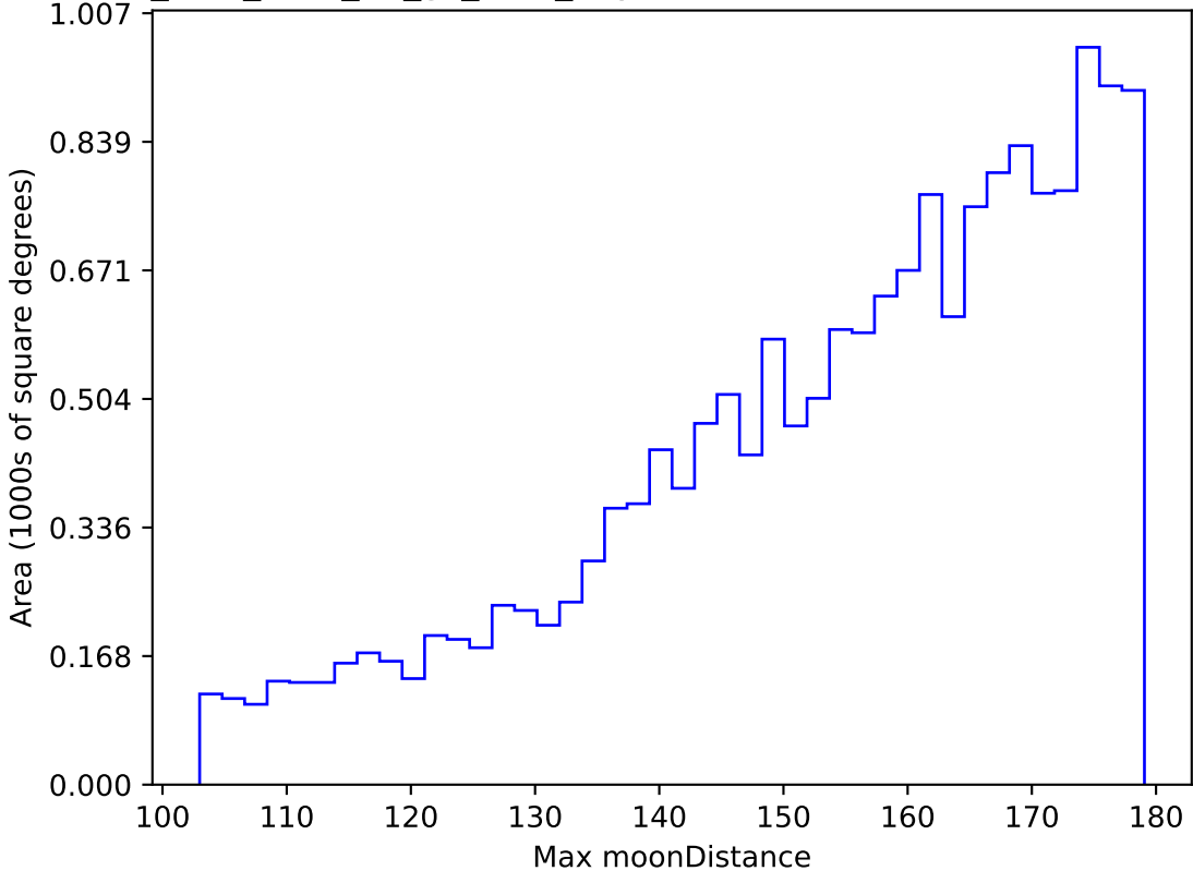
too_elab_r128_d2_gz_v3.4_10yrs WFD z band: Max moonDistance
