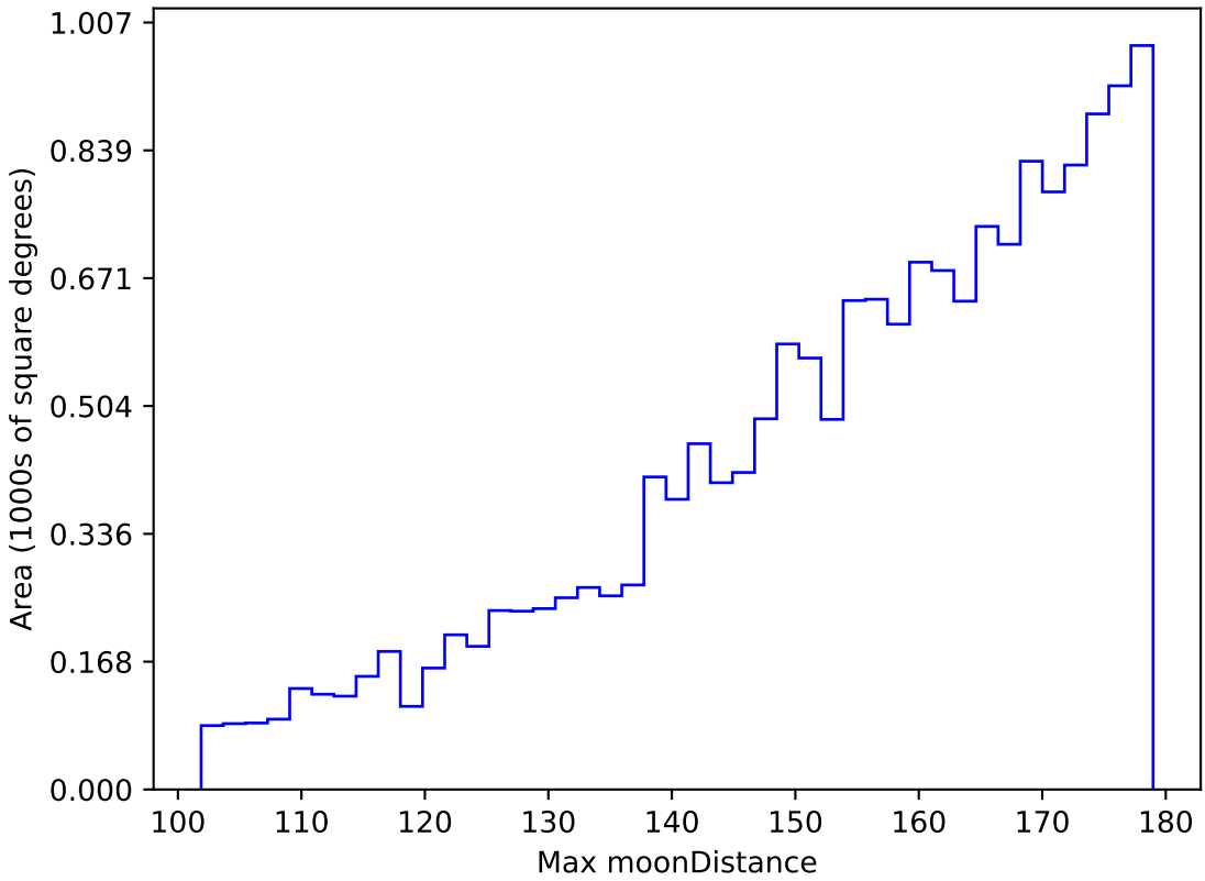
too_elab_r128_d2_gz_v3.4_10yrs WFD u band: Max moonDistance
