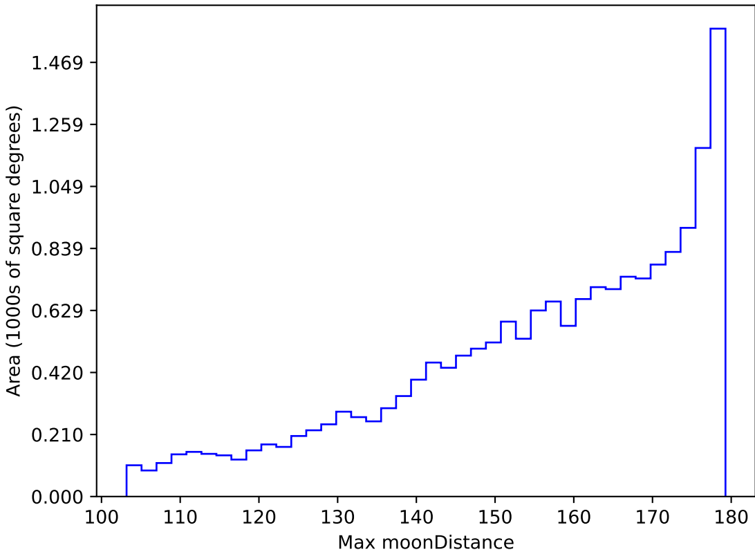
too_elab_r128_d2_gz_v3.4_10yrs WFD r band: Max moonDistance
