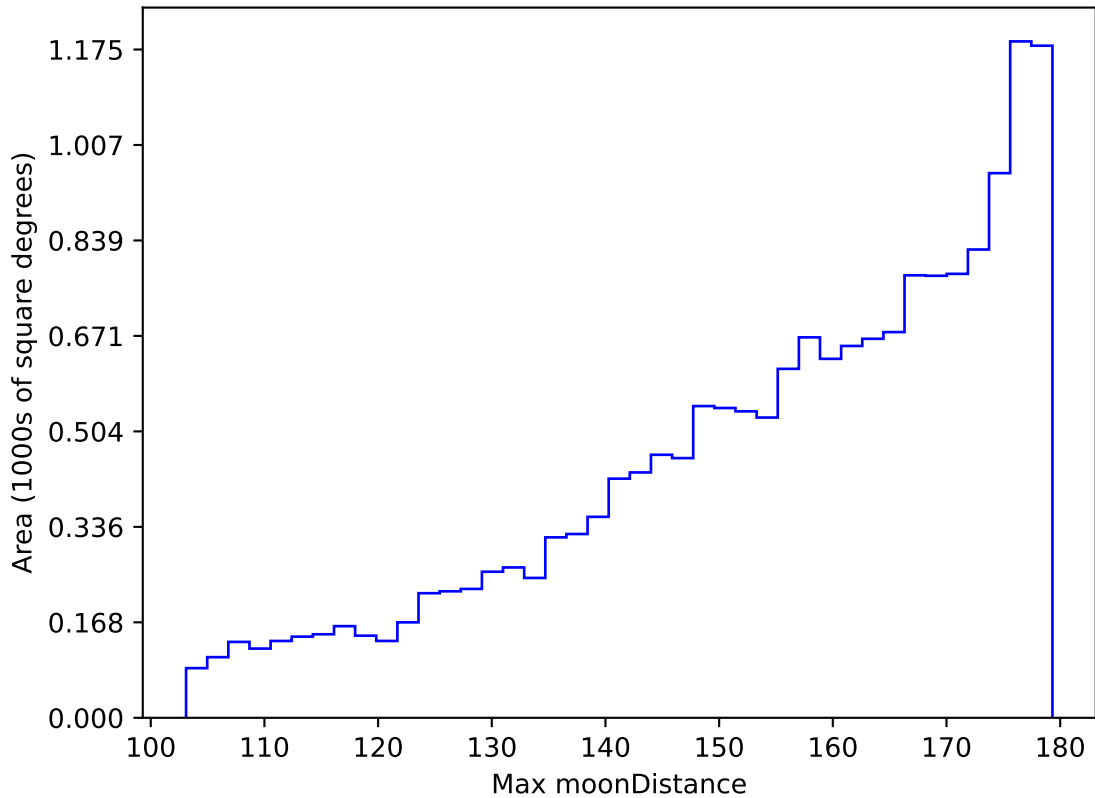
too_elab_r128_d2_gz_v3.4_10yrs WFD i band: Max moonDistance
