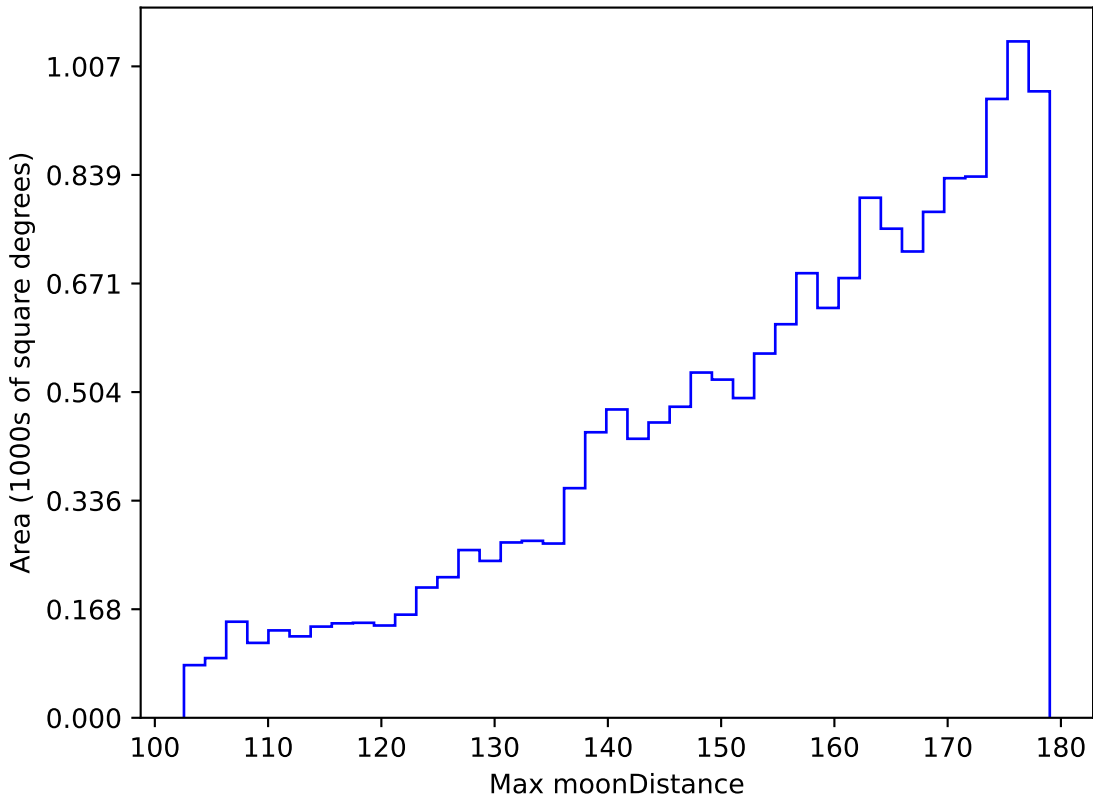
too_elab_r128_d2_gz_v3.4_10yrs WFD g band: Max moonDistance
