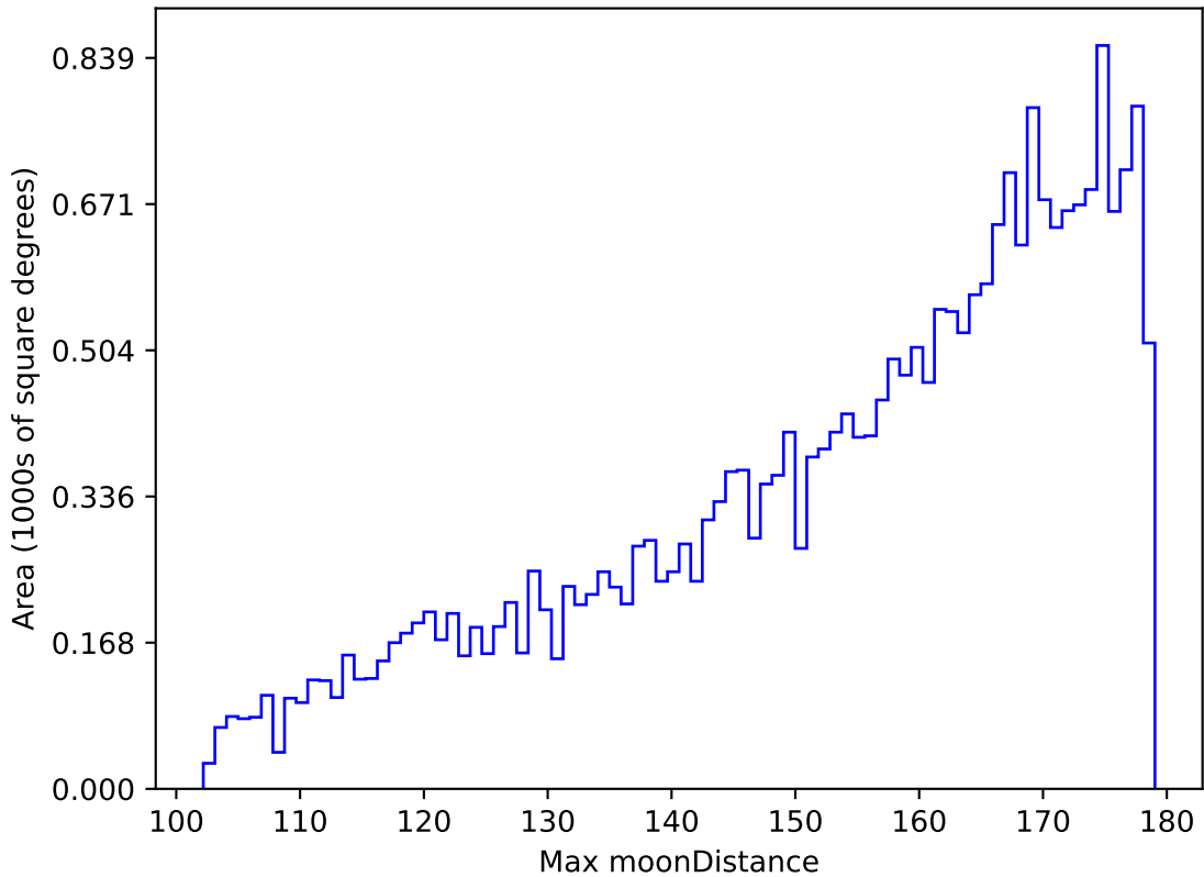
too_elab_r128_d2_gz_v3.4_10yrs All sky z band: Max moonDistance
