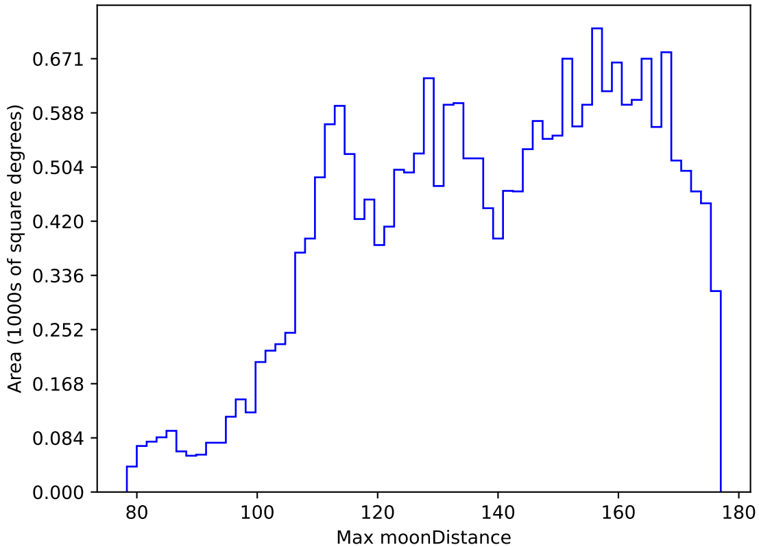
too_elab_r128_d2_gz_v3.4_10yrs All sky y band: Max moonDistance
