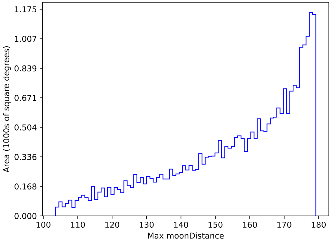
too_elab_r128_d2_gz_v3.4_10yrs All sky r band: Max moonDistance
