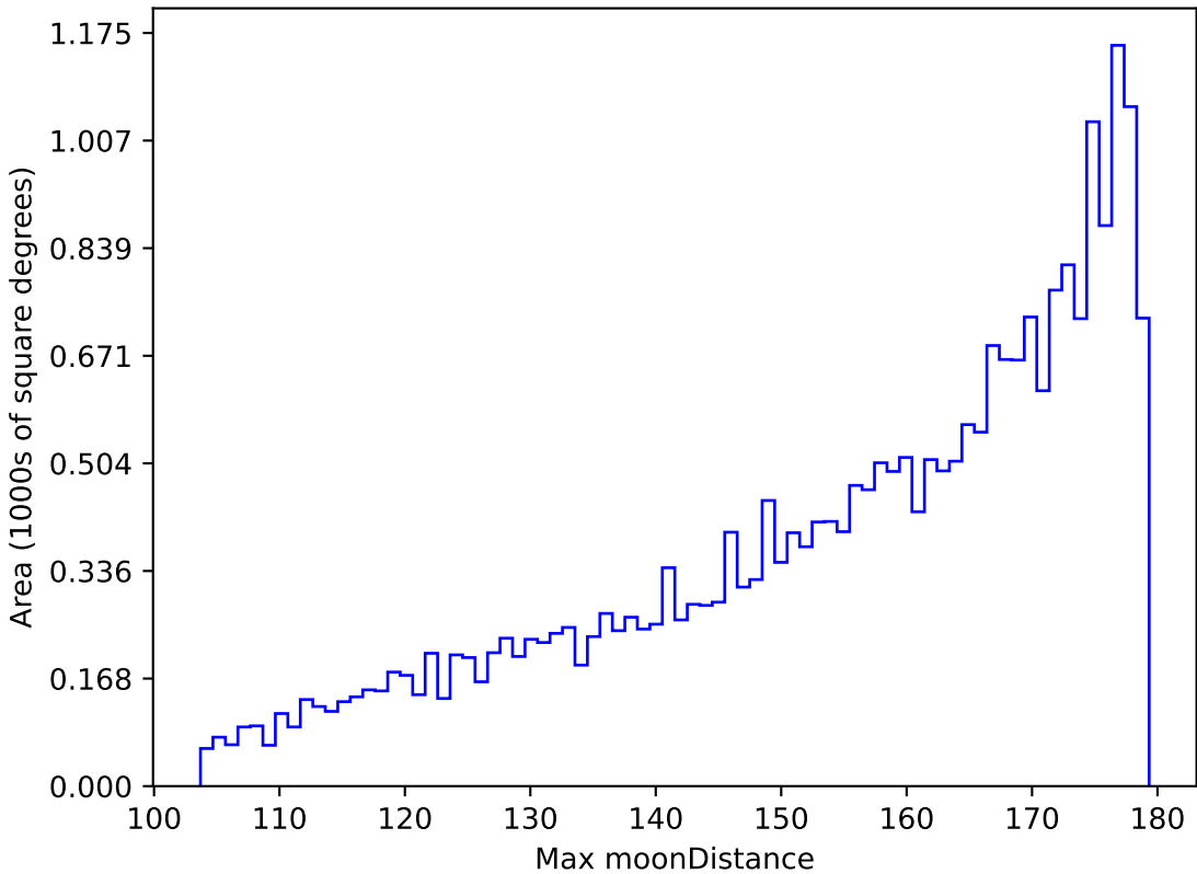
too_elab_r128_d2_gz_v3.4_10yrs All sky i band: Max moonDistance
