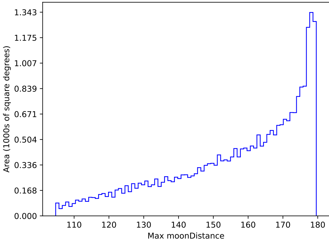
too_elab_r128_d2_gz_v3.4_10yrs All sky all bands: Max moonDistance
