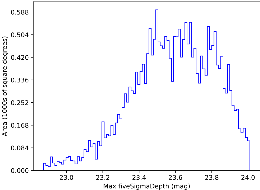
too_elab_r128_d2_gz_v3.4_10yrs Yr 1 u band: Max fiveSigmaDepth
