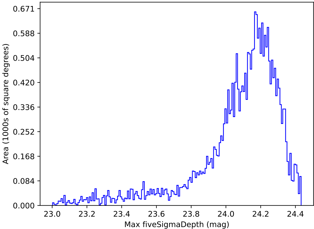
too_elab_r128_d2_gz_v3.4_10yrs Yr 1 i band: Max fiveSigmaDepth
