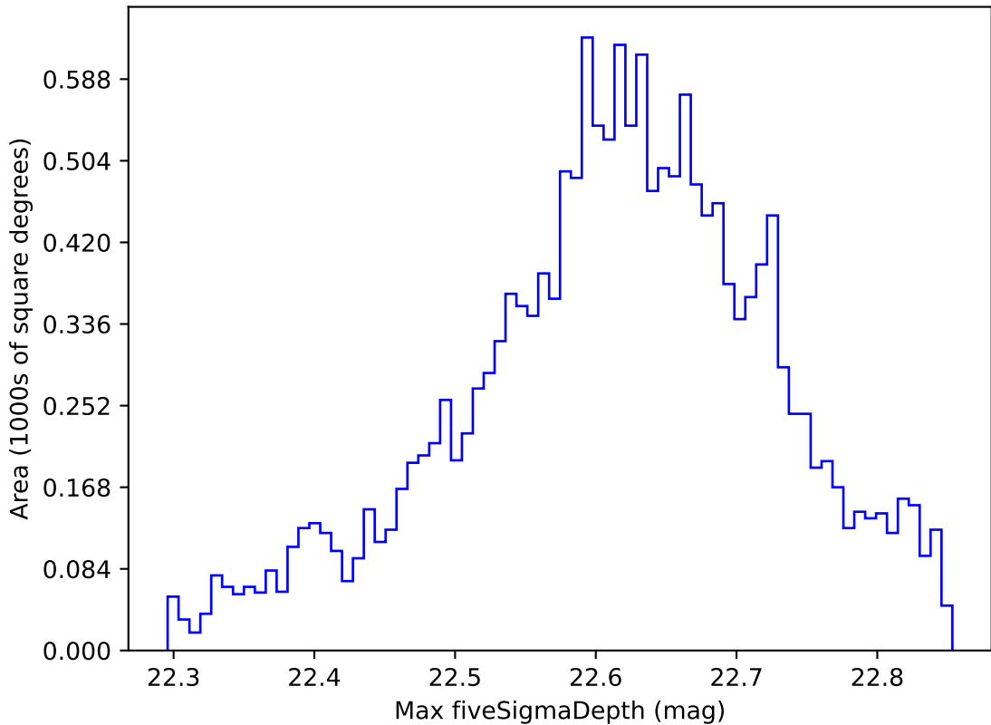
too_elab_r128_d2_gz_v3.4_10yrs WFD y band: Max fiveSigmaDepth
