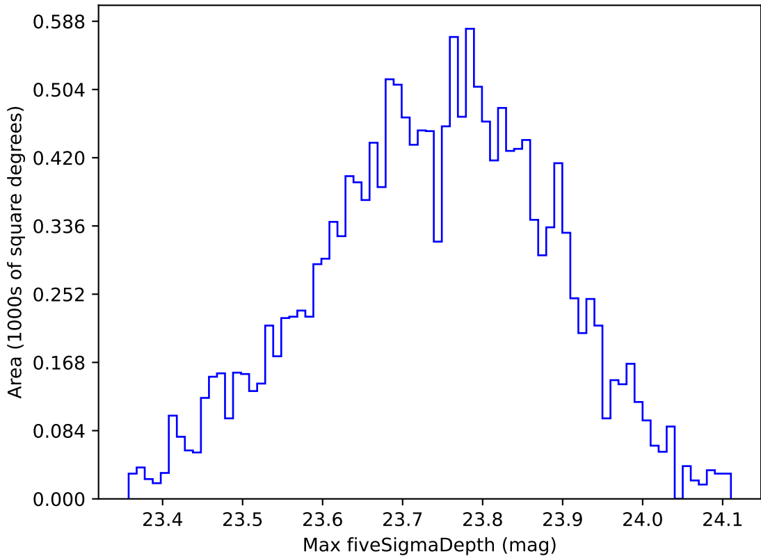
too_elab_r128_d2_gz_v3.4_10yrs WFD u band: Max fiveSigmaDepth
