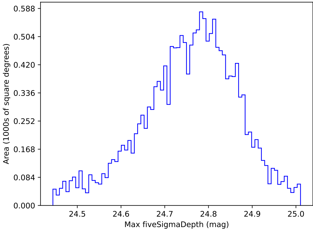
too_elab_r128_d2_gz_v3.4_10yrs WFD r band: Max fiveSigmaDepth
