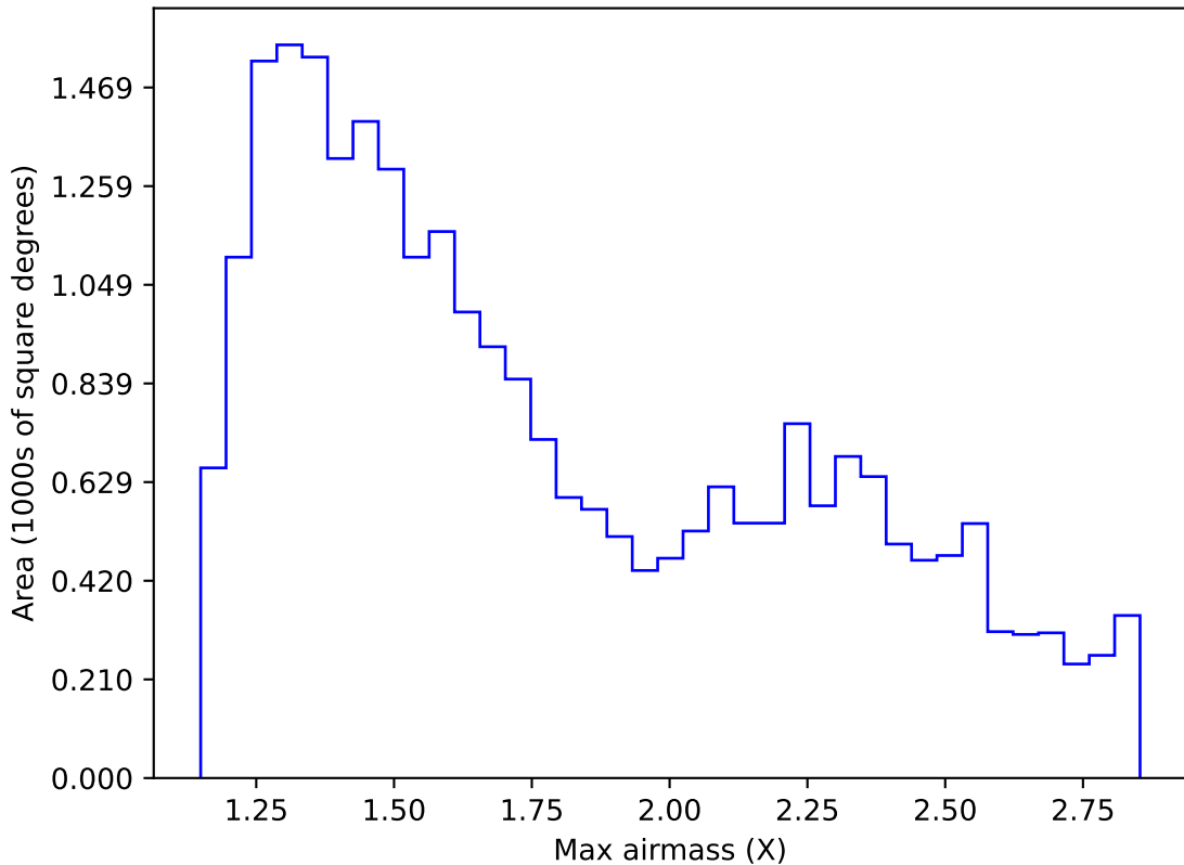
too_elab_r128_d2_gz_v3.4_10yrs Yr 1 i band: Max airmass
