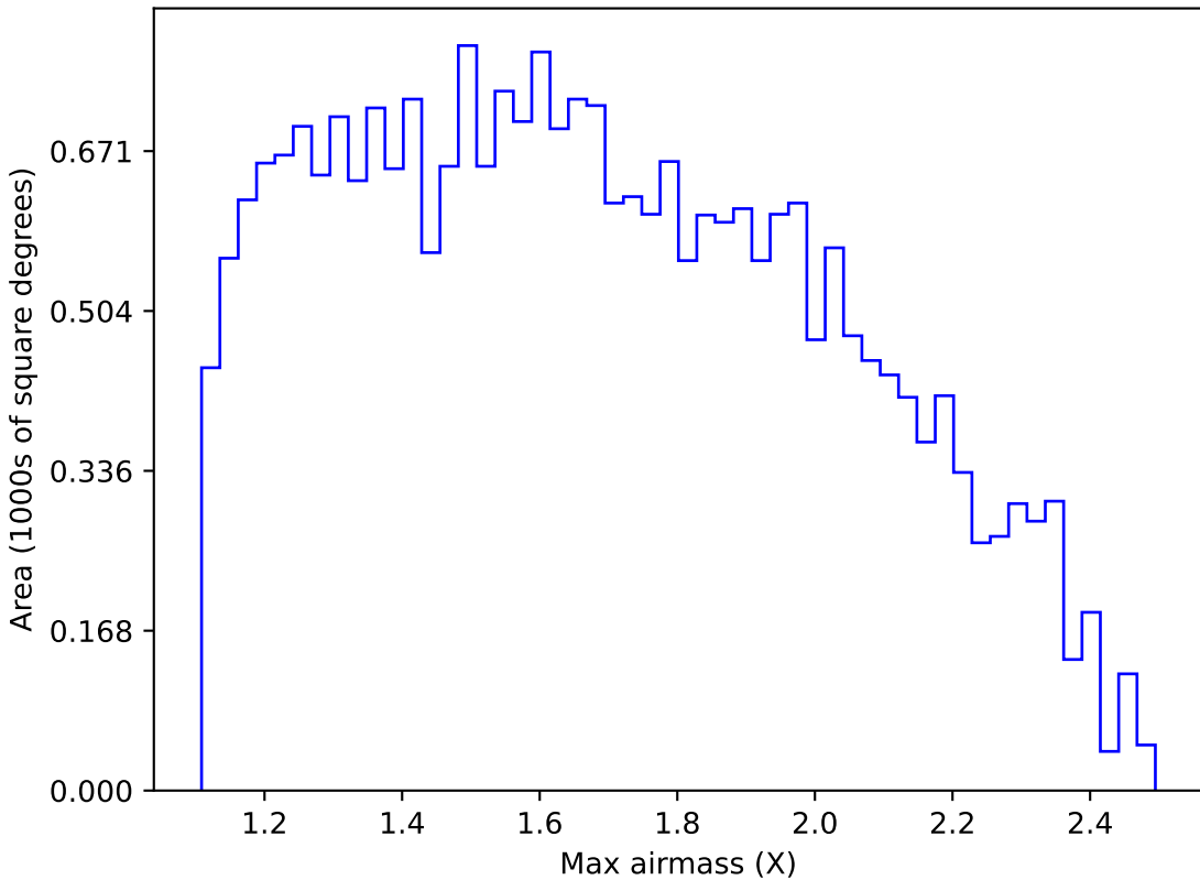
too_elab_r128_d2_gz_v3.4_10yrs Yr 1 g band: Max airmass
