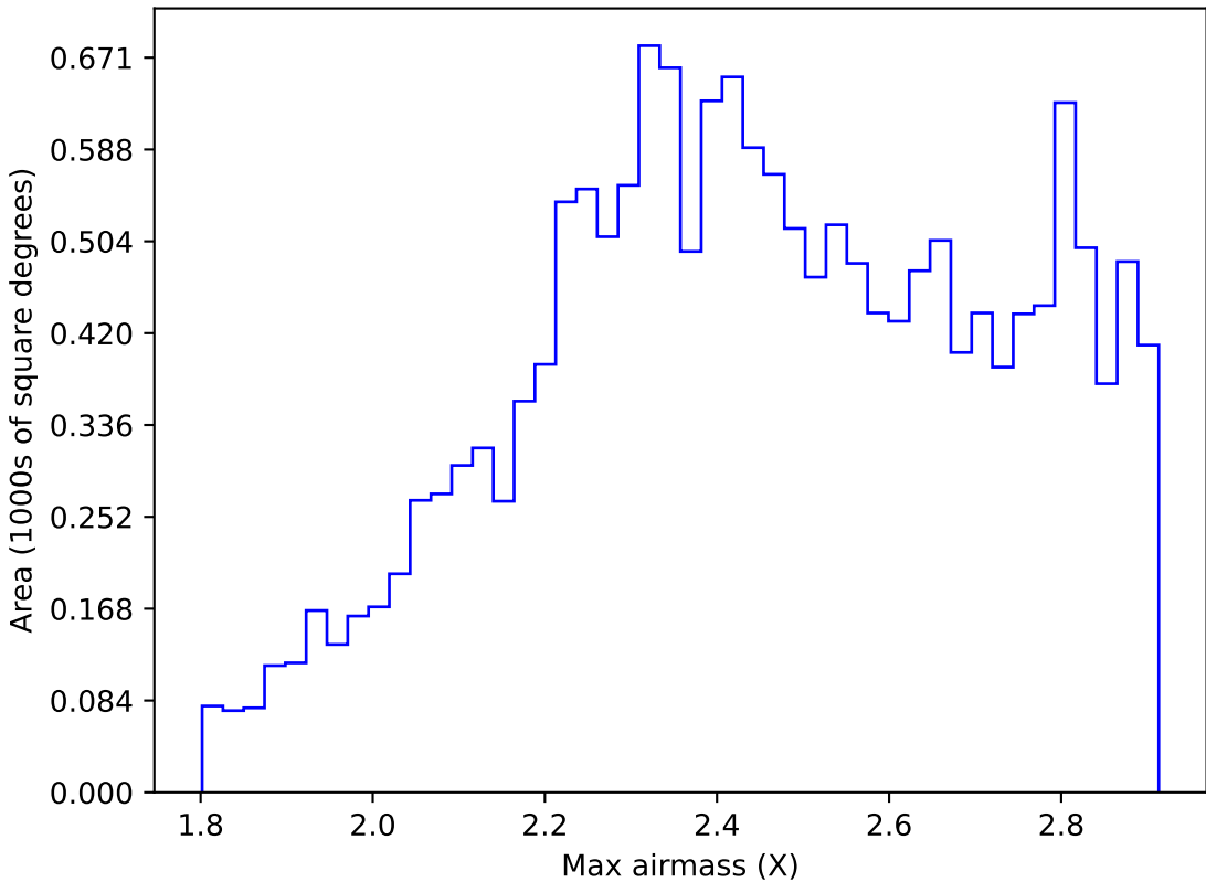
too_elab_r128_d2_gz_v3.4_10yrs WFD z band: Max airmass
