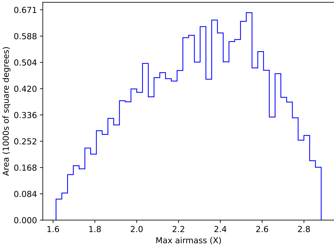
too_elab_r128_d2_gz_v3.4_10yrs WFD y band: Max airmass
