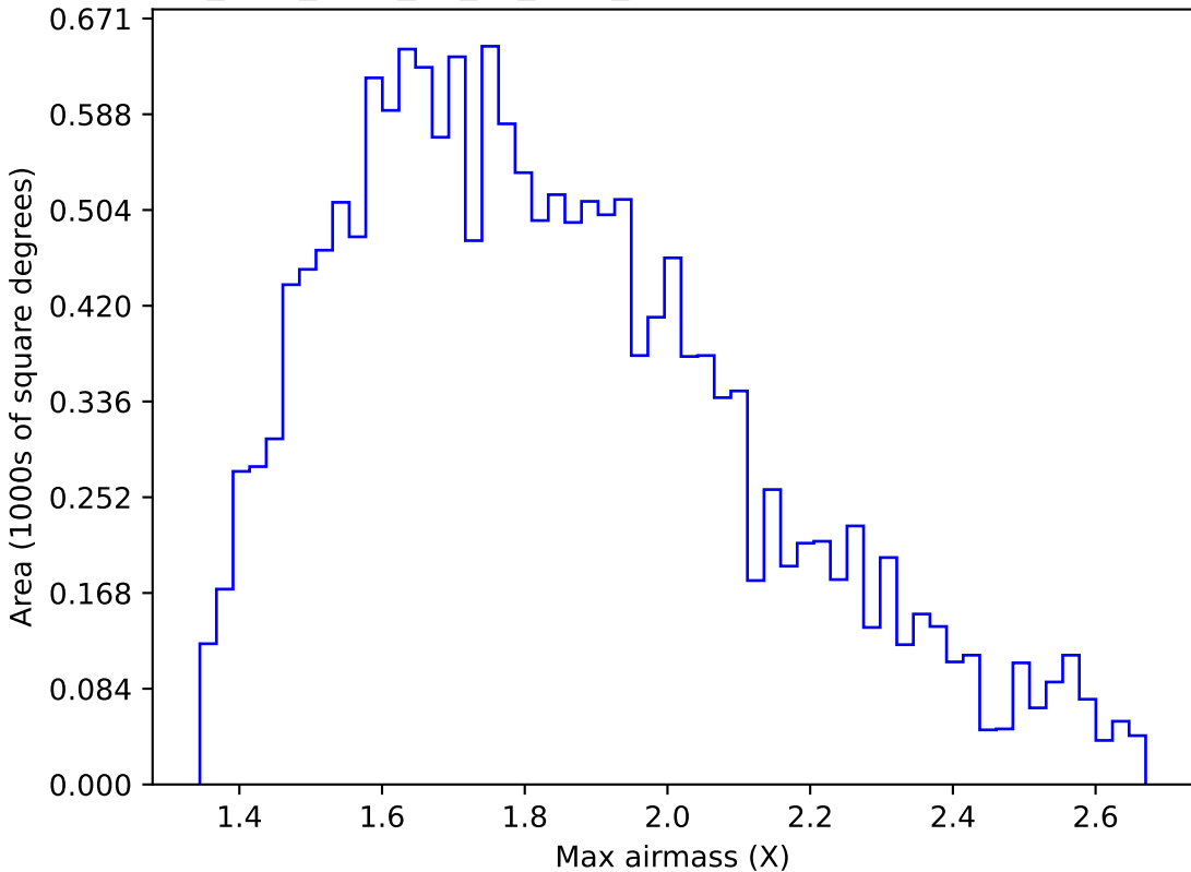
too_elab_r128_d2_gz_v3.4_10yrs WFD u band: Max airmass
