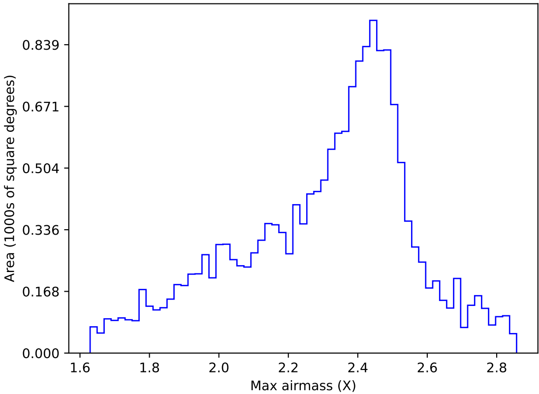
too_elab_r128_d2_gz_v3.4_10yrs WFD r band: Max airmass
