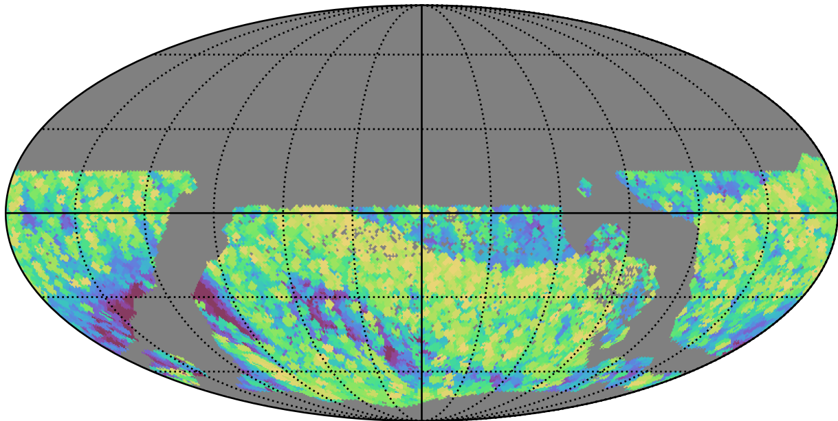
too_elab_r128_d2_gz_v3.4_10yrs WFD all bands: Max airmass
