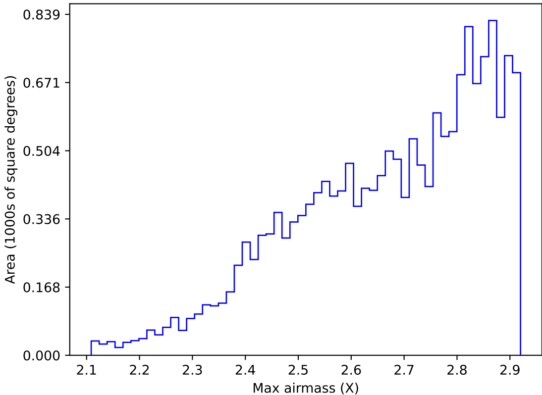
too_elab_r128_d2_gz_v3.4_10yrs WFD all bands: Max airmass
