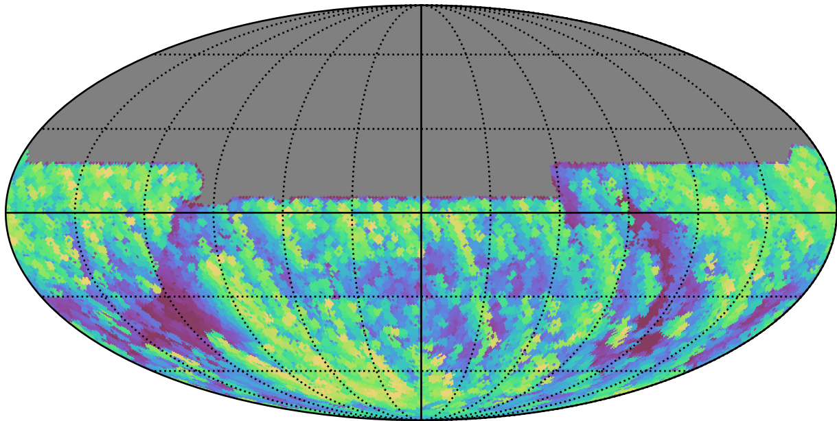
too_elab_r128_d2_gz_v3.4_10yrs All sky y band: Max airmass
