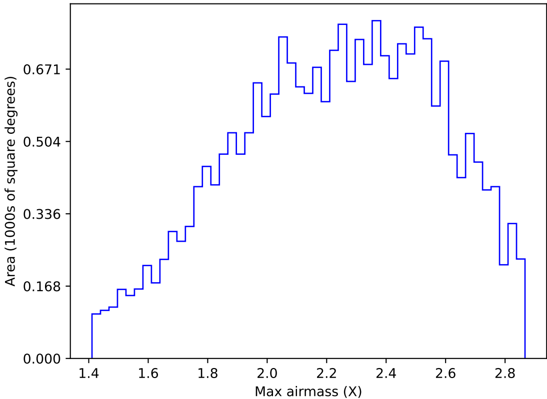
too_elab_r128_d2_gz_v3.4_10yrs All sky y band: Max airmass
