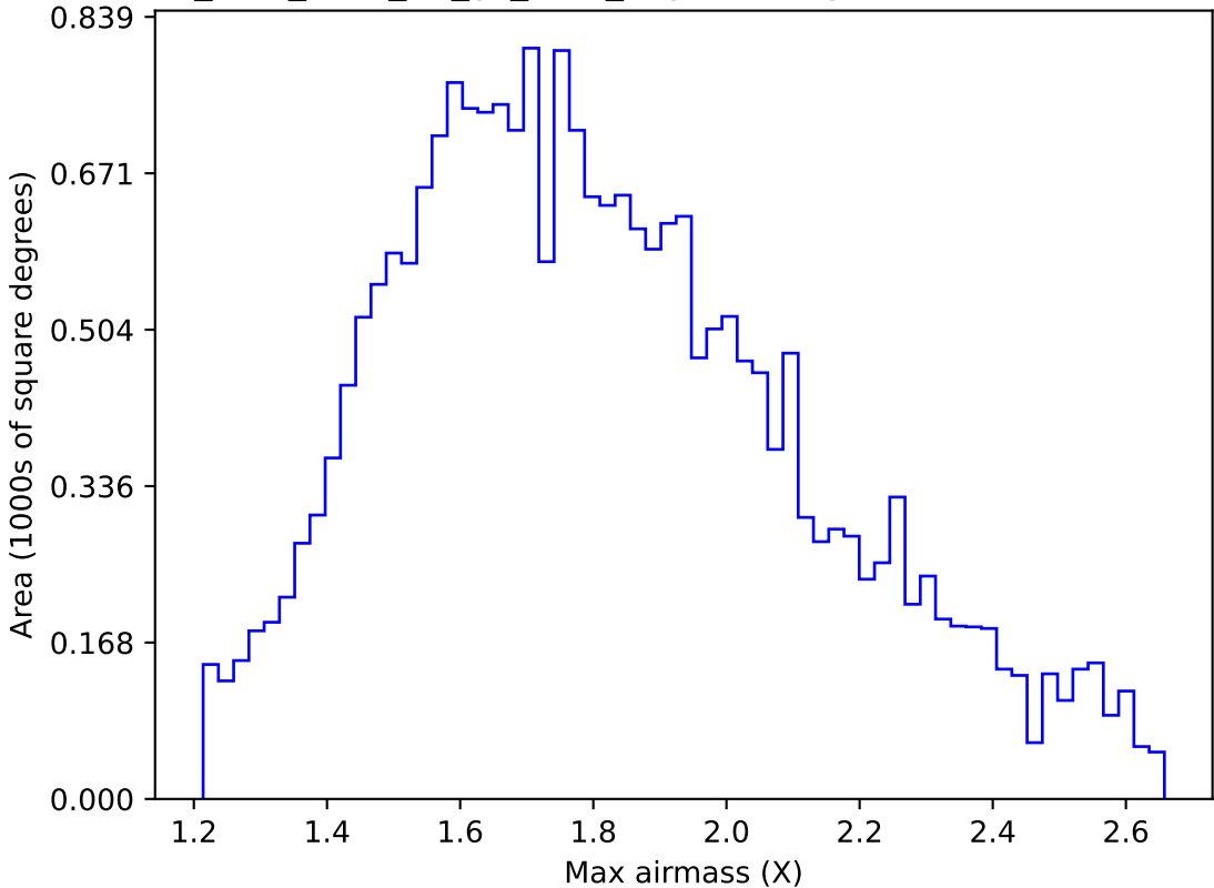
too_elab_r128_d2_gz_v3.4_10yrs All sky u band: Max airmass
