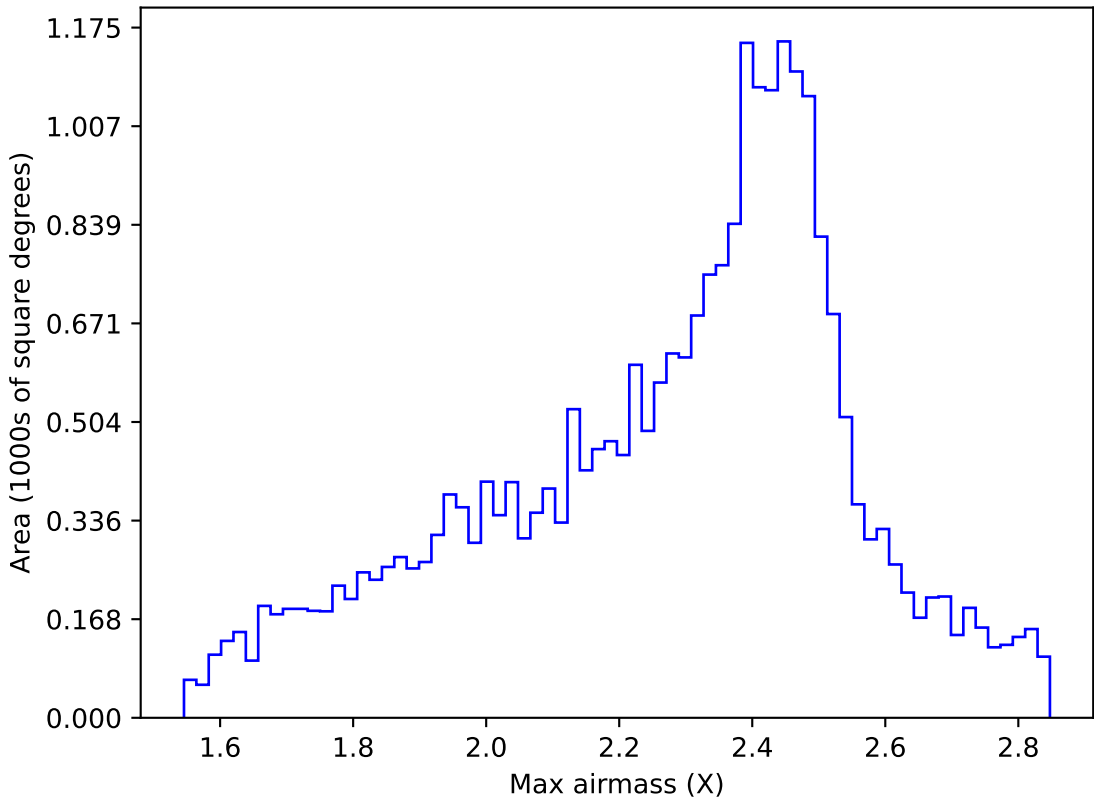
too_elab_r128_d2_gz_v3.4_10yrs All sky r band: Max airmass
