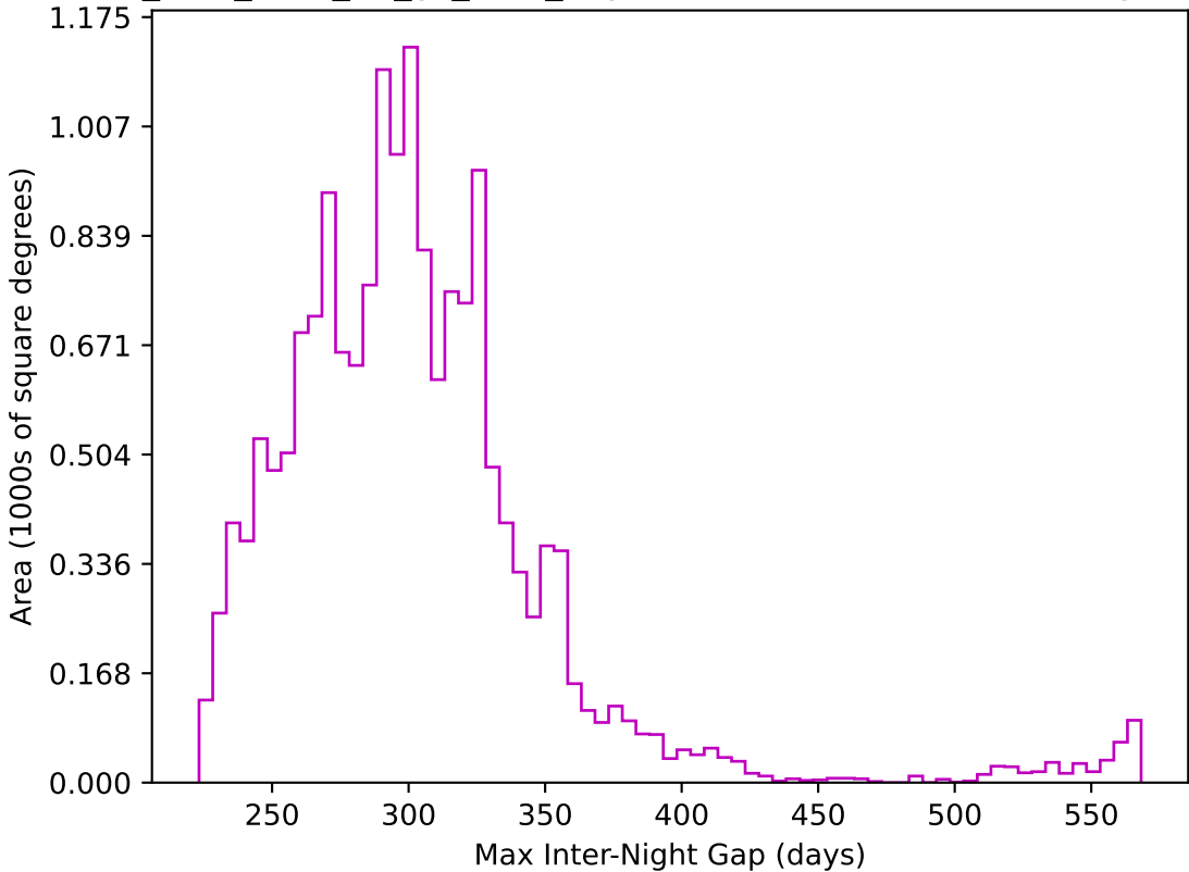
too_elab_r128_d2_gz_v3.4_10yrs WFD z band: Max Inter-Night Gap
