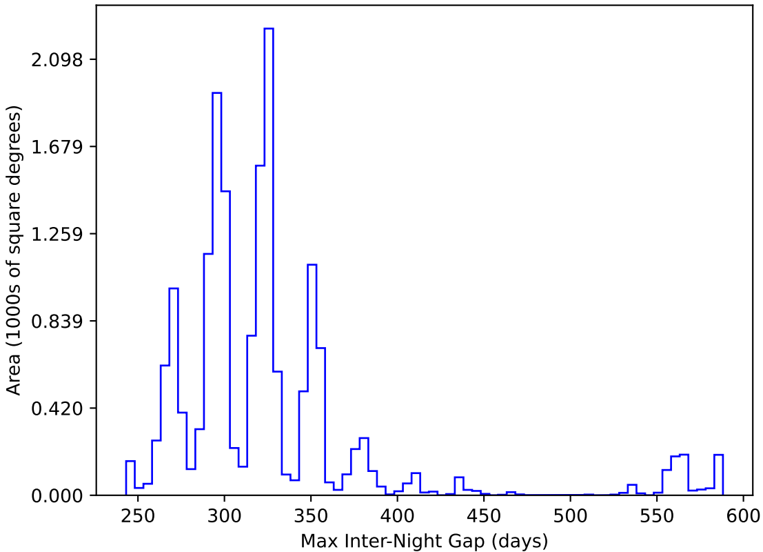
too_elab_r128_d2_gz_v3.4_10yrs WFD y band: Max Inter-Night Gap
