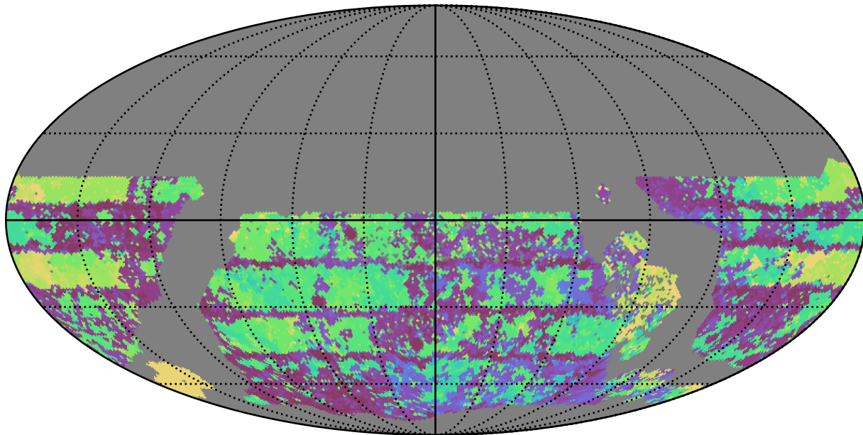
too_elab_r128_d2_gz_v3.4_10yrs WFD u band: Max Inter-Night Gap
