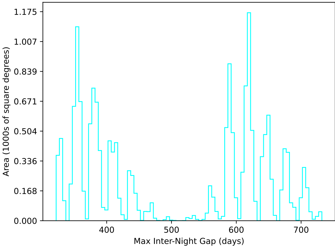
too_elab_r128_d2_gz_v3.4_10yrs WFD u band: Max Inter-Night Gap
