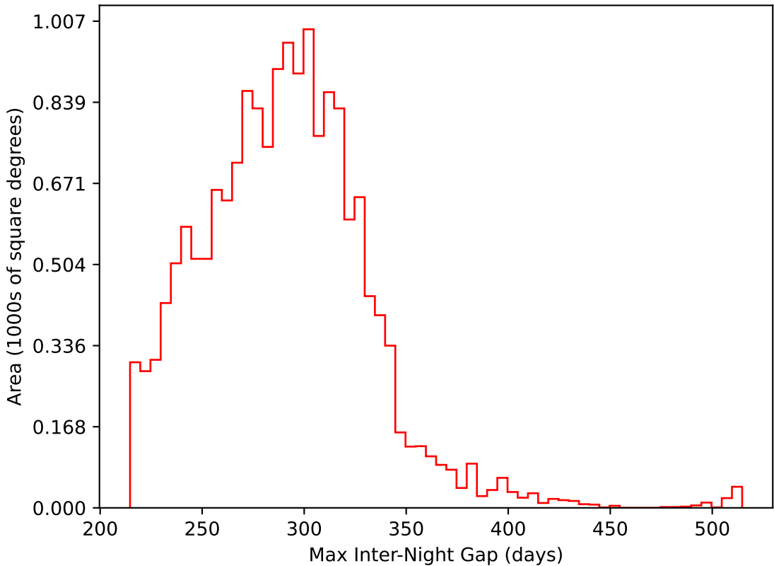
too_elab_r128_d2_gz_v3.4_10yrs WFD i band: Max Inter-Night Gap
