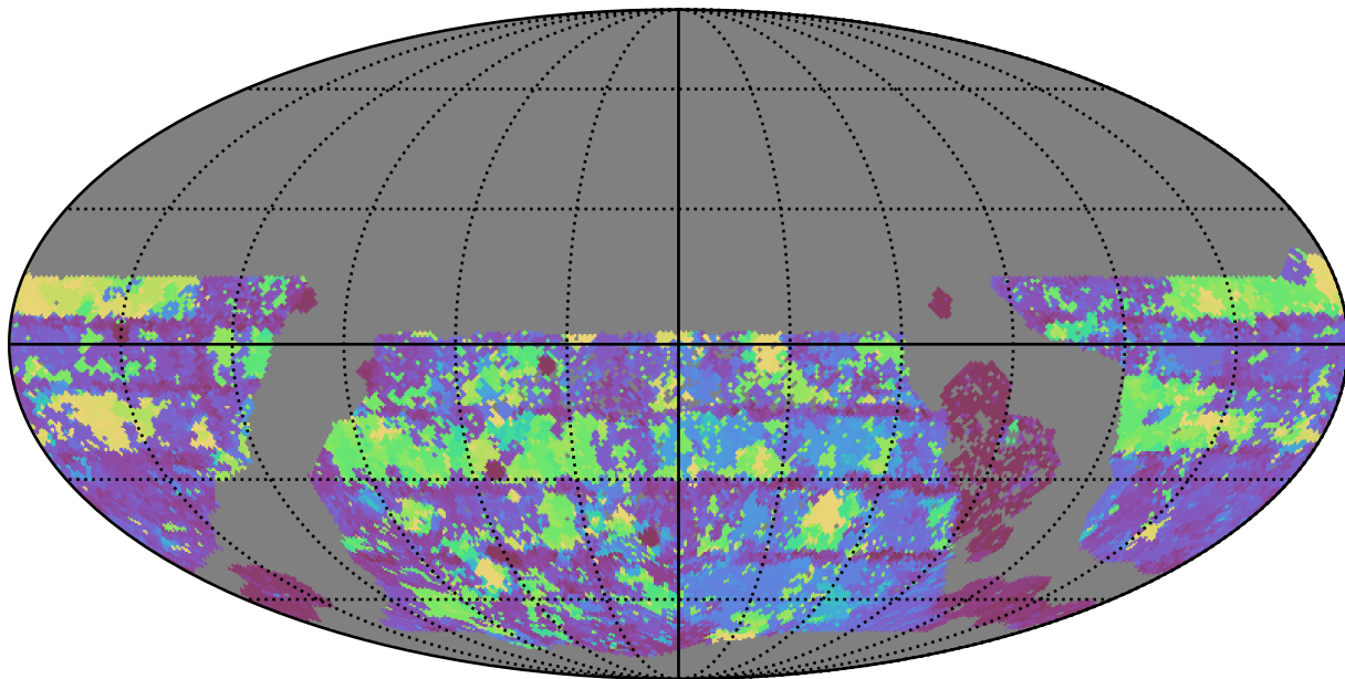
too_elab_r128_d2_gz_v3.4_10yrs WFD g band: Max Inter-Night Gap
